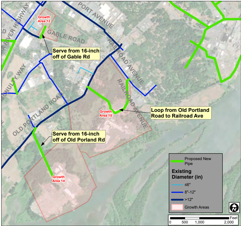
FIGURE 5-12: GROWTH AREA 12, 14, AND 15 PROPOSED PIPING
